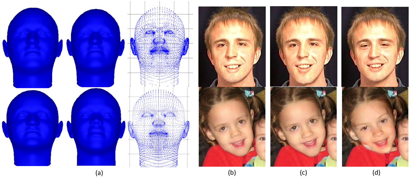
Figure 10: Comparisons with other methods. (a). 3D Models and the difference flows generated by FaceGen Modeller. (b). Composites generated using FaceGen models. (c). Composites generated using the single image fitting algorithm (Algorithm 1). (d). Whole face replacement results. Compared with our results in Figure 1 and 8, these results contain more severe artifacts.
